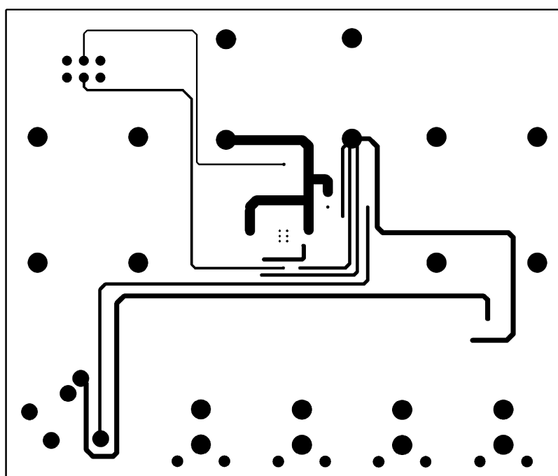
FIGURE 6. Bottom Layer
