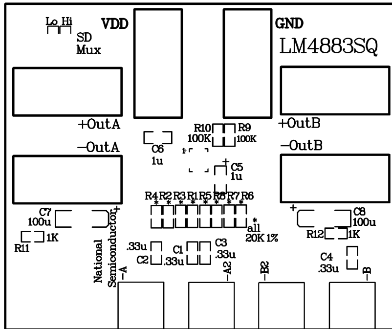
FIGURE 7. Silkscreen
